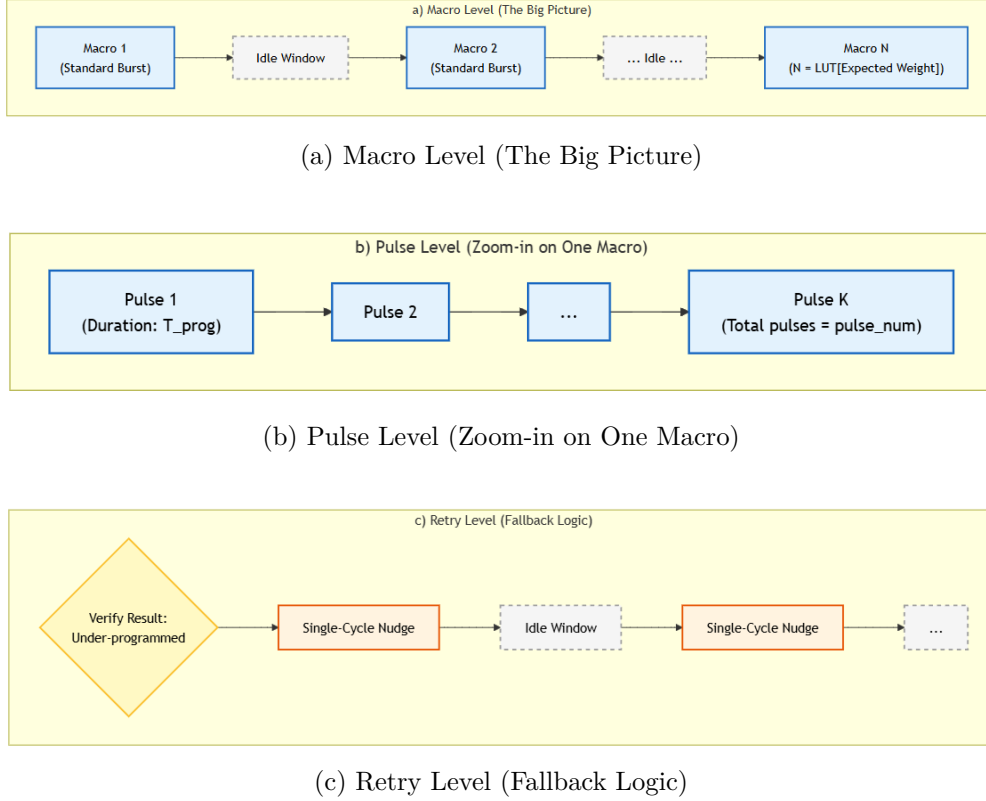
Figure 4.11: LUT-based macro-repeat structure for the programming attempts. (a) For the first attempt, the controller concatenates a number of macros given by the LUT entry for the expected weight, separated by idle windows. (b) The inner macro detail, showing one standard burst of discrete pulses. (c) Retry attempts on the same cell switch to a single-cycle nudge train, on the assumption that the first attempt has already moved the cell most of the way to the target.
