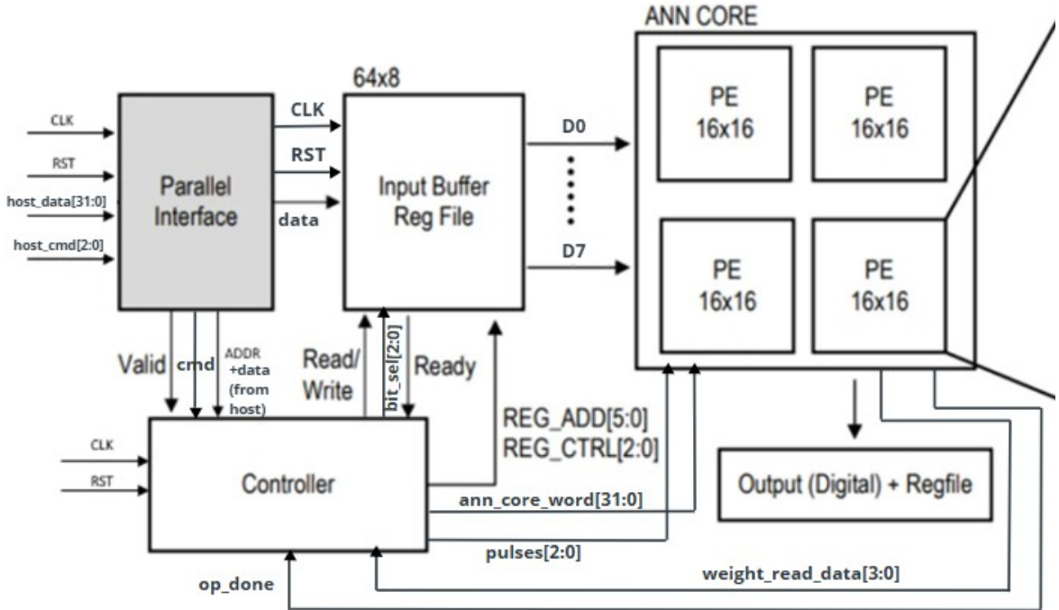
Figure 3.1: Top-level block diagram. The host drives a transaction word and a command token into the combinational Parallel Interface , which qualifies the packet and produces a validated bus consumed by the ANN Controller . The controller sequences commands toward the analog ANN core over a packed core word and a pulse-mode bus, and it simultaneously drives the Input Buffer that stores inference pixels and the expected-weight nibble used during verify. A single status bit from the core ( op_done ) closes the loop in the program and erase sub-FSMs.
