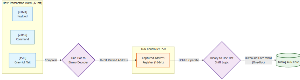
Figure 3.2: Pictorial layout of the 32-bit transaction word and the internal round-trip used by the controller: the host one-hot tail is decoded into a 16-bit packed binary address, the FSM captures and operates on the packed address, and the outbound core word is rebuilt by single-bit left-shifts into the one-hot domain just before reaching the core.
