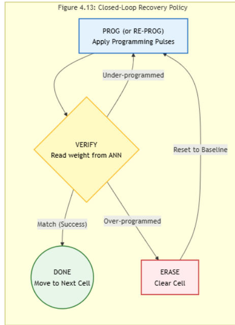
Figure 4.13: Closed-loop recovery policy. The \text{PROG} \rightarrow \text{VERIFY} \rightarrow \text{ERASE} \rightarrow \text{RE-PROG} loop maps every analog failure mode to a deterministic digital recovery path.
