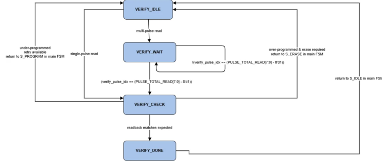
Figure 4.8: CHECK state branching logic: match, under-programmed, over-programmed. The three outcomes drive the closed-loop recovery policy — success returns to idle, under-programmed retries (or falls back to erase when the per-cell retry budget is exhausted), and over-programmed triggers an erase followed by reprogramming.
