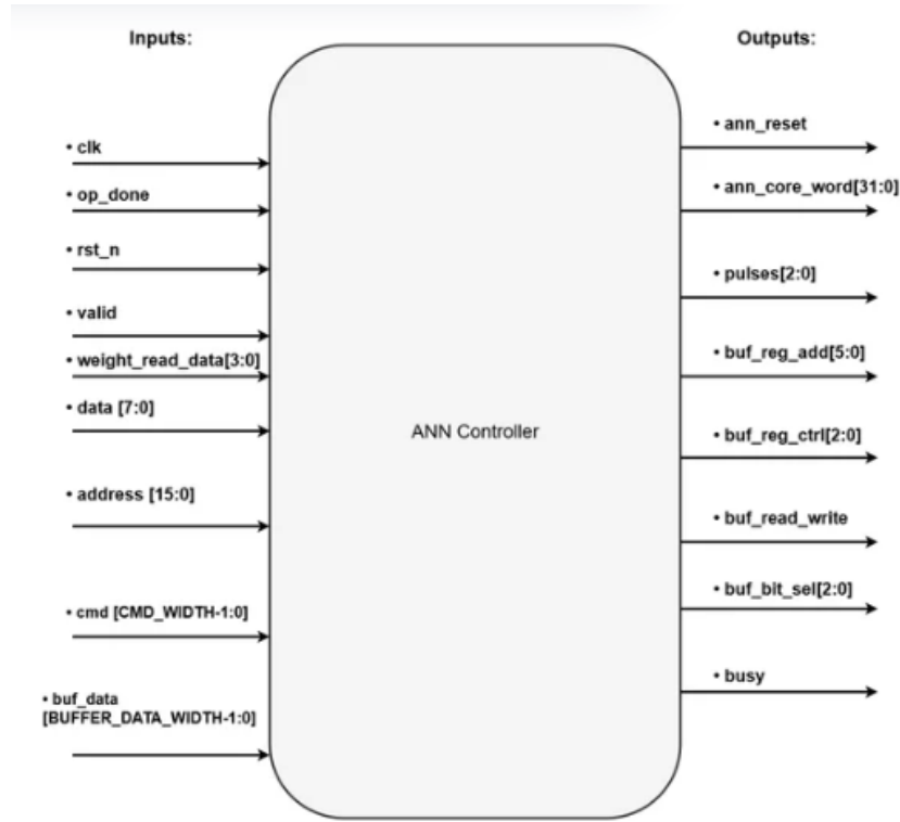
Figure 4.4: ANN Controller I/O block diagram. Host-side inputs ( address , data , cmd , valid ) arrive pre-validated from the parallel interface; analog-side inputs ( op_done , weight_read_data ) close the program/erase and verify loops. The controller emits the packed core word ( addr_out , data_out ), the three-bit pulse-mode bus ( pulses ), the buffer-control port set, and a small bank of status flags ( erase_retry_exhausted , verify_failed ).
