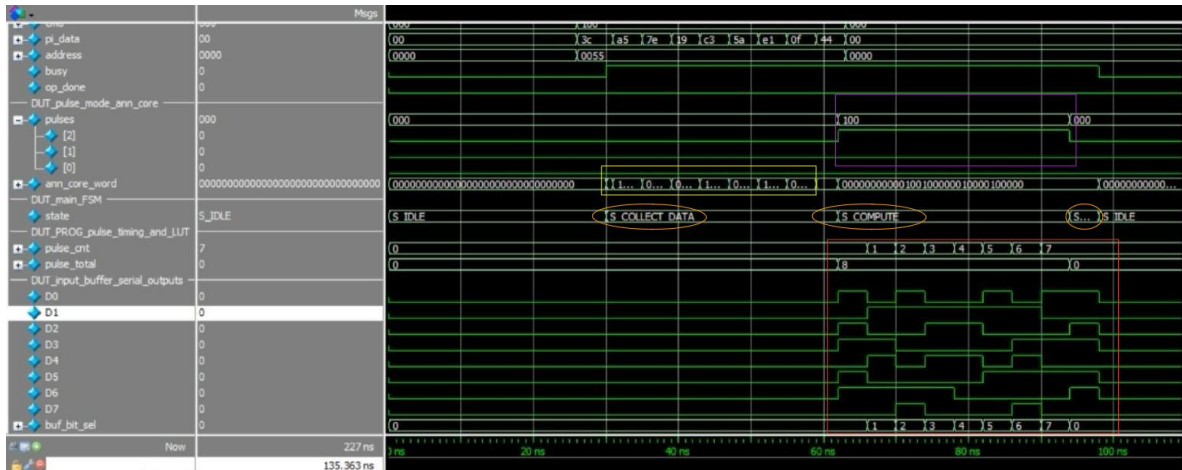
Figure 6.4: Inference dataflow (Transaction overview): The top-level sequence of the inference command, annotated to show the FSM progressing linearly through S_COLLECT_DATA \rightarrow S_COMPUTE \rightarrow S_IDLE .
